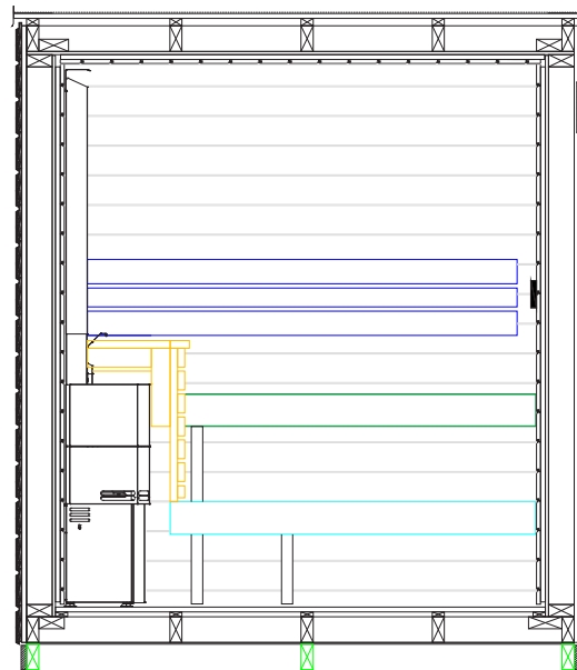
SECTION 2-2
