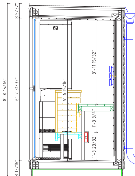
SECTION 1-1
