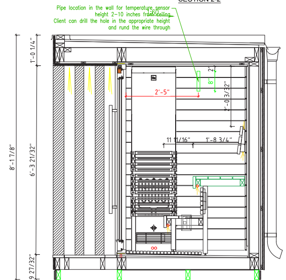
SECTION 2-2
