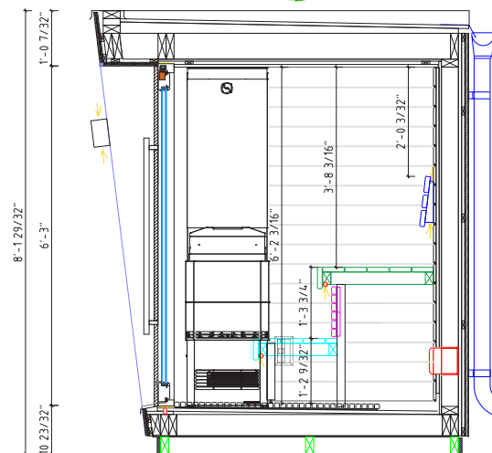
SECTION 2-2
